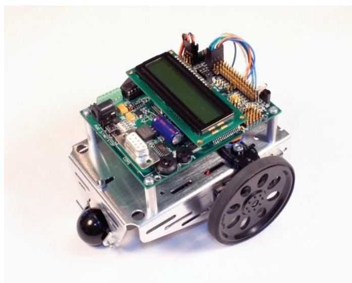
Slika 2.2 IntelliBrain-Bot robot basic oprema
